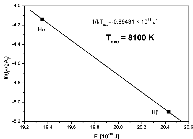
Figure 15. Determination of the excitational temperature from the relative intensities of atomic hydrogen lines \text{H}_\alpha and \text{H}_\beta of the Balmer series.
