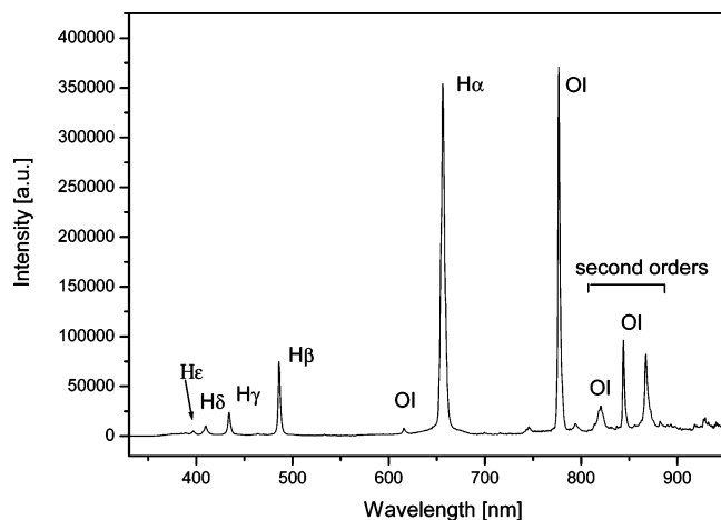
Figure 5. Optical emission spectrum of LIDB in water vapor.
